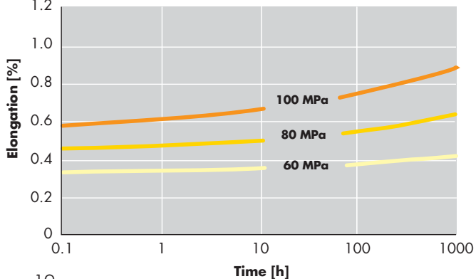
Creep curves for Grivory GVX-5H at 23°C/50% r.h.
